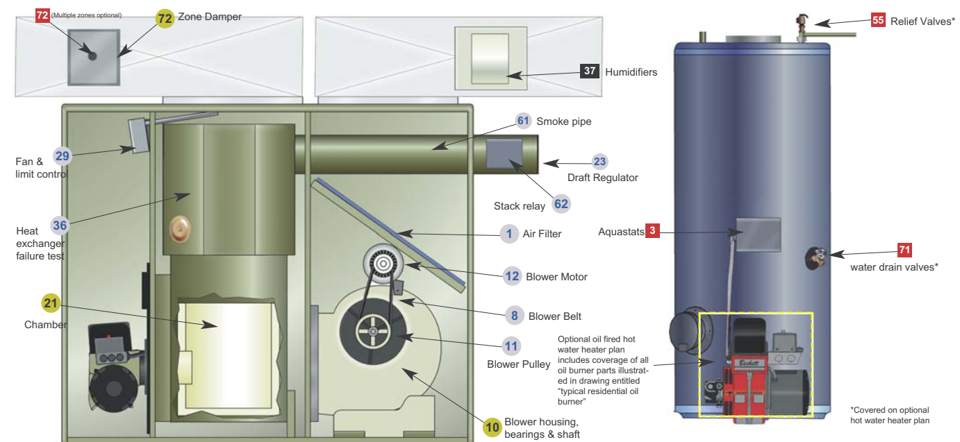
Typical Residential Warm Air Furnace
