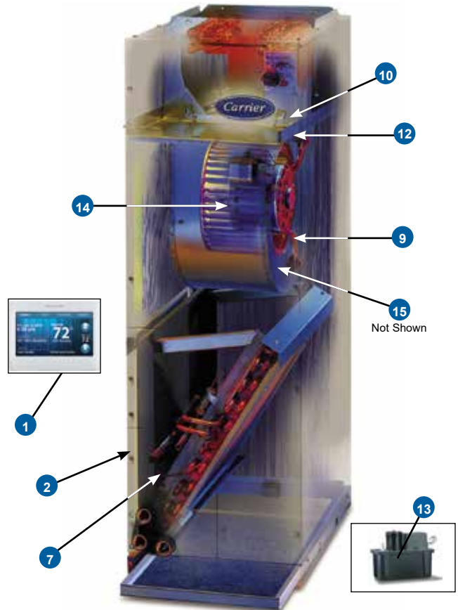
Typical Air Handling Unit
