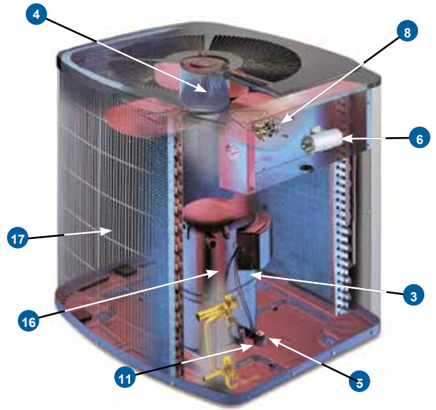
Typical Condensing Unit
